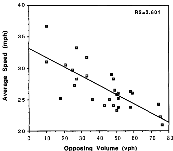
Figure 4. Average Speed vs. Opposing Traffic Volume
