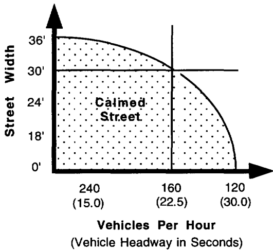
Figure 10. Calmed Street Hypothesis
