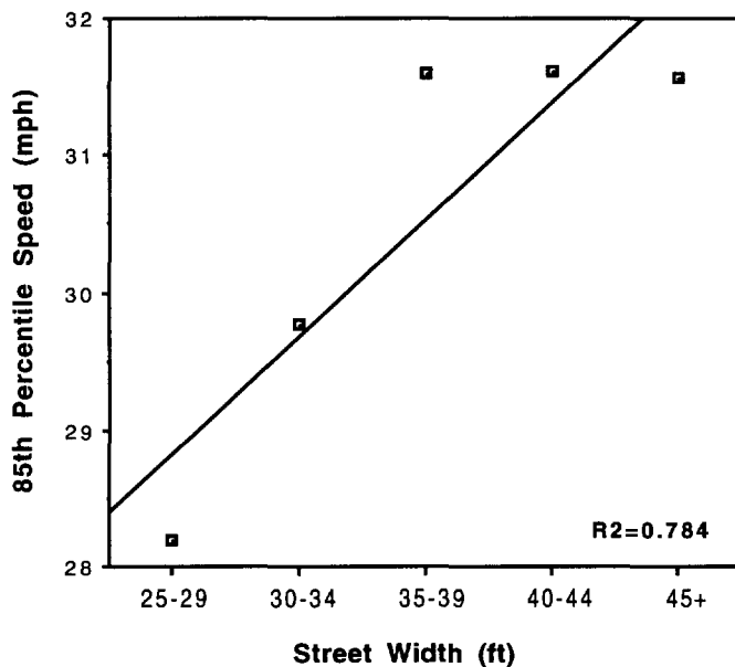
Figure 3. 85th Percentile Speed vs. Street Width Group
